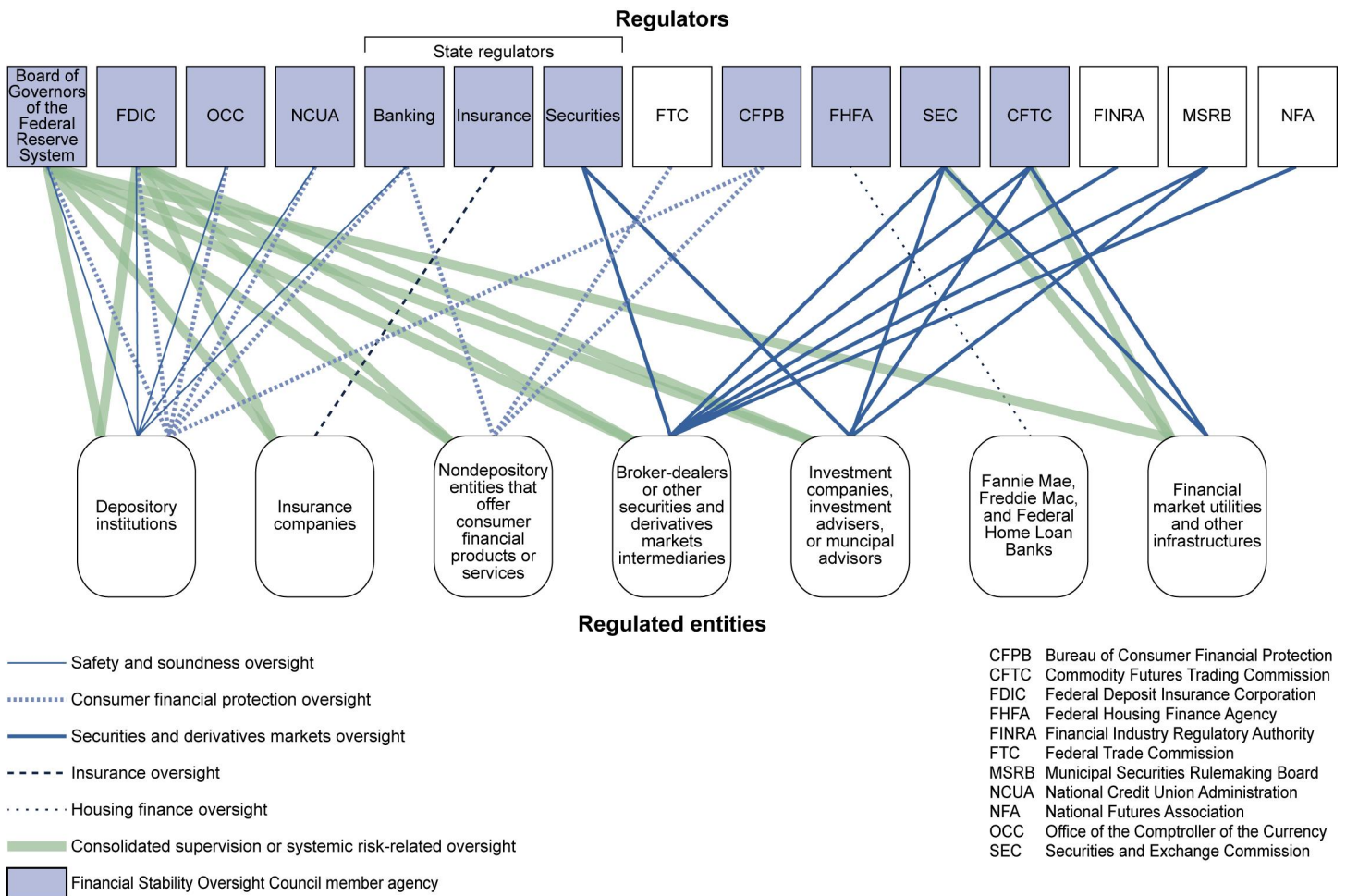
Figure 2: U.S. Financial Regulatory Structure, 2016
