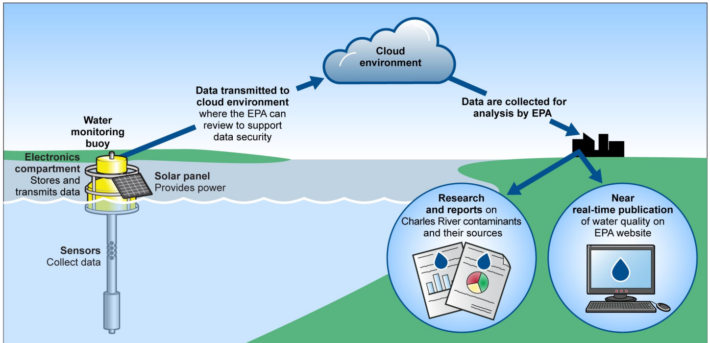
Figure 2: Environmental Protection Agency (EPA) Buoy That Uses Internet of Things Technologies to Remotely Monitor Water Quality in the Charles River
