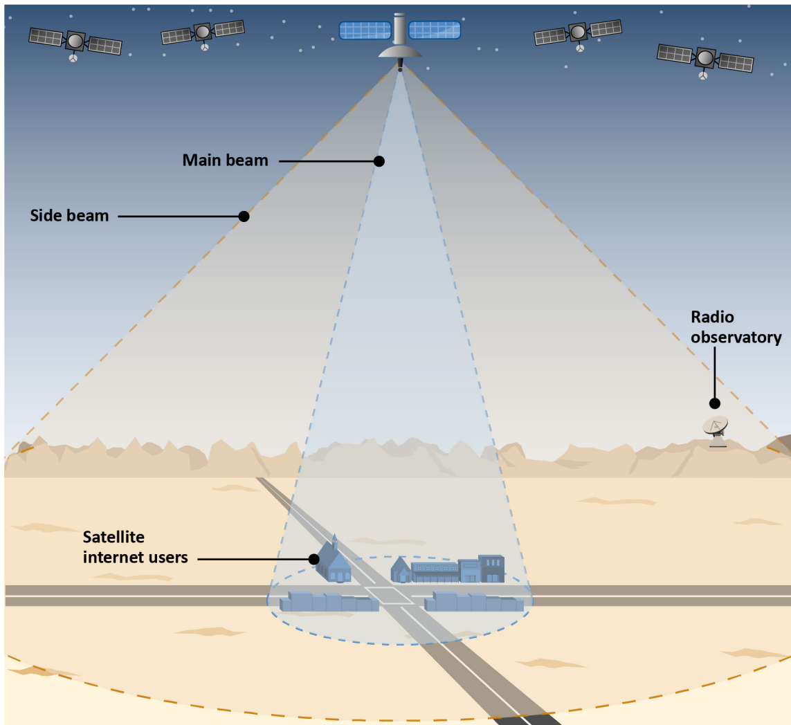
Figure 8: Satellite effects for radio astronomy: Side beam transmissions
