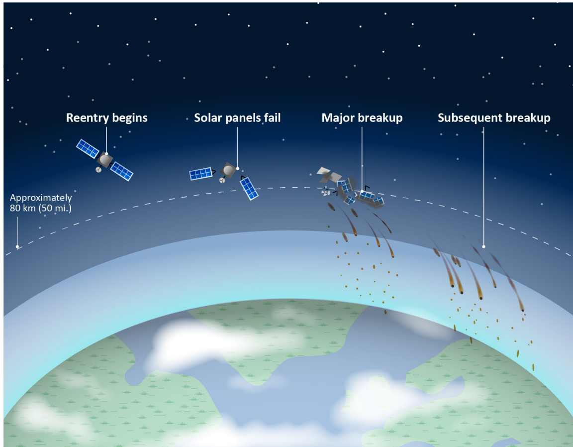
Figure 5: Satellite reentry and breakup
