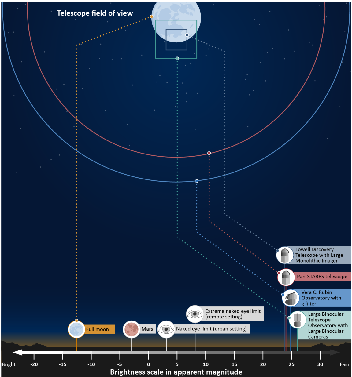
Figure 7: Brightness of astronomical objects, sensitivity of telescopes, and telescope fields of view compared to the moon
