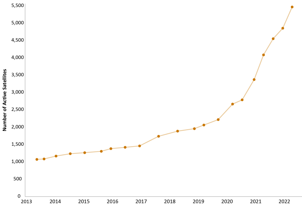
Figure 2: Approximate number of active satellites, 2013-2022
