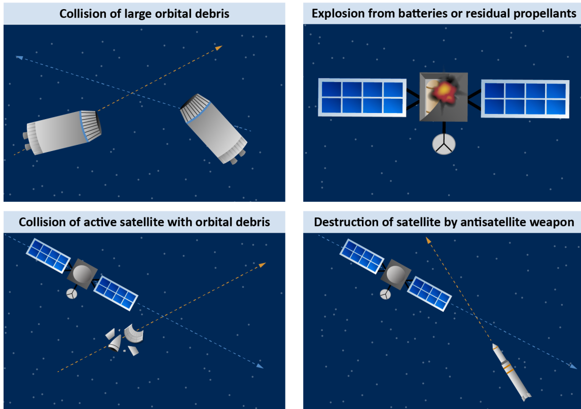
Figure 9: Orbital debris can come from various sources
