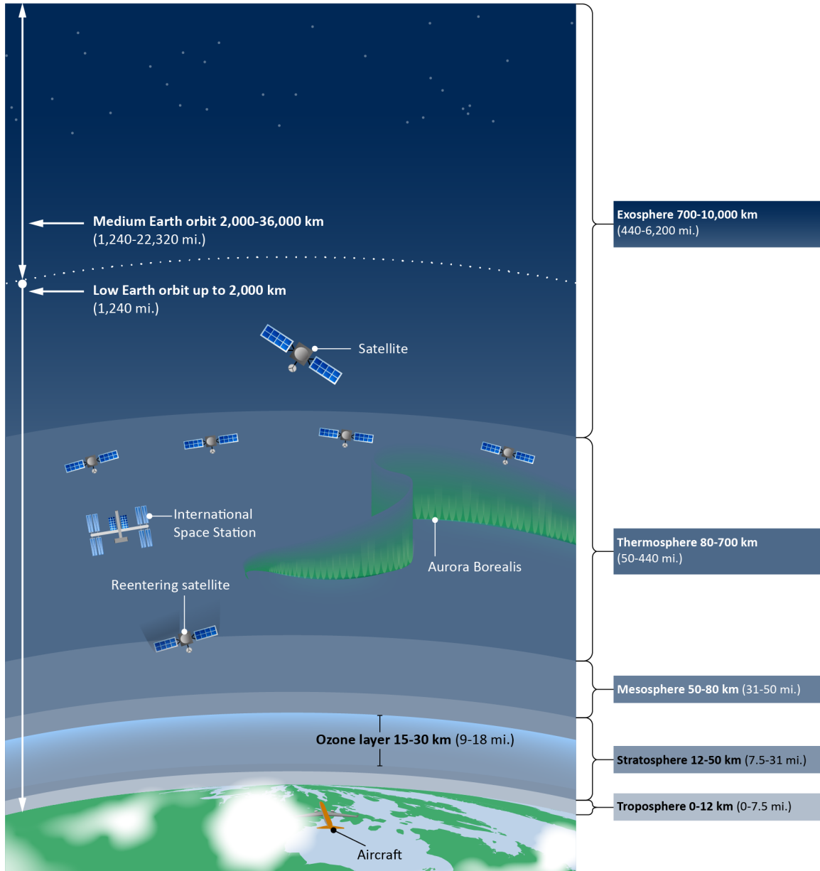
Figure 4: Layers of the Earth's atmosphere
