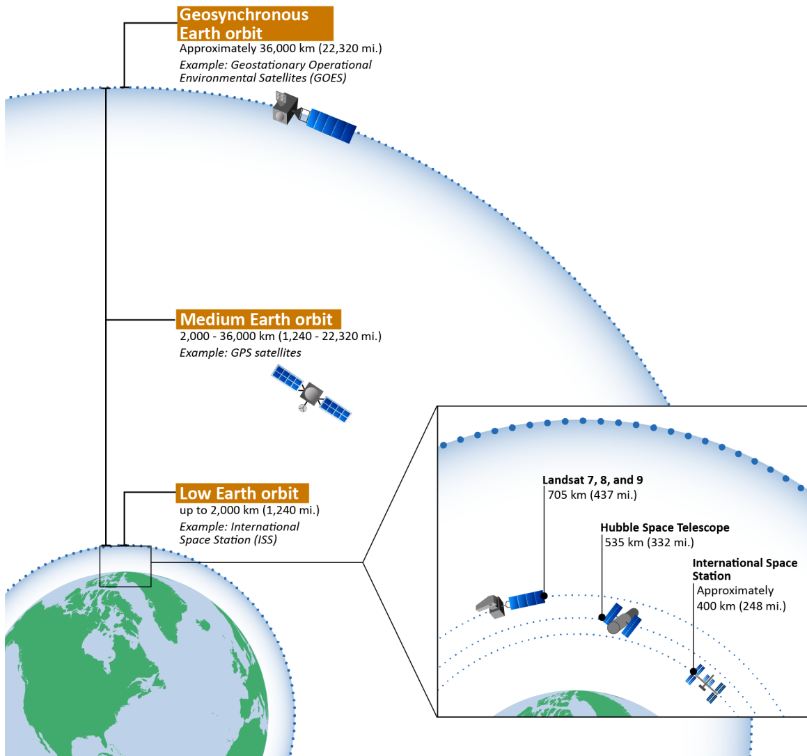
Figure 1: Categories of Earth orbits with reference spacecraft
