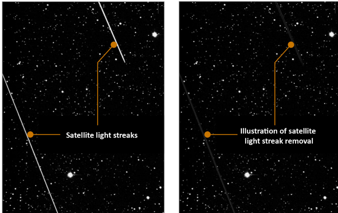
Figure 6: Light streaks from large constellations of satellites in an optical astronomy image
