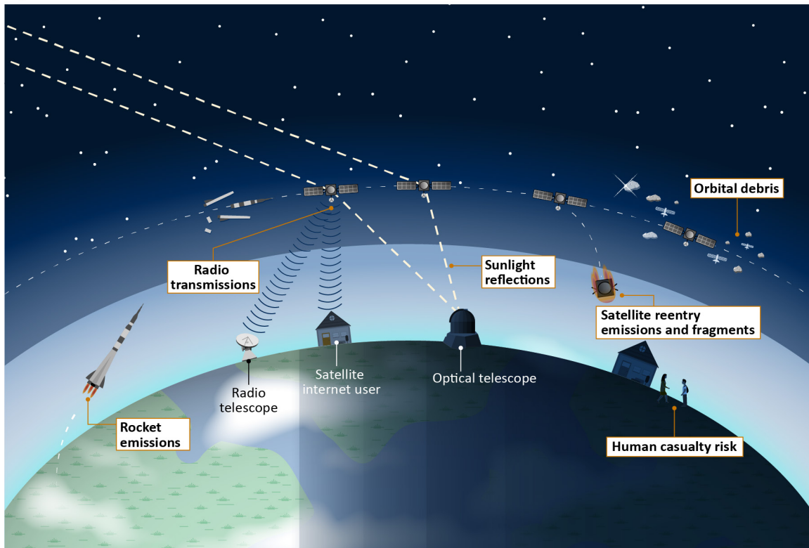
Figure 3: Categories of environmental and other effects of constellations of satellites
