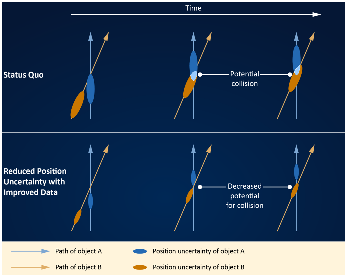
Figure 11: Reduced uncertainties in the positioning of space objects can decrease the potential of a collision
