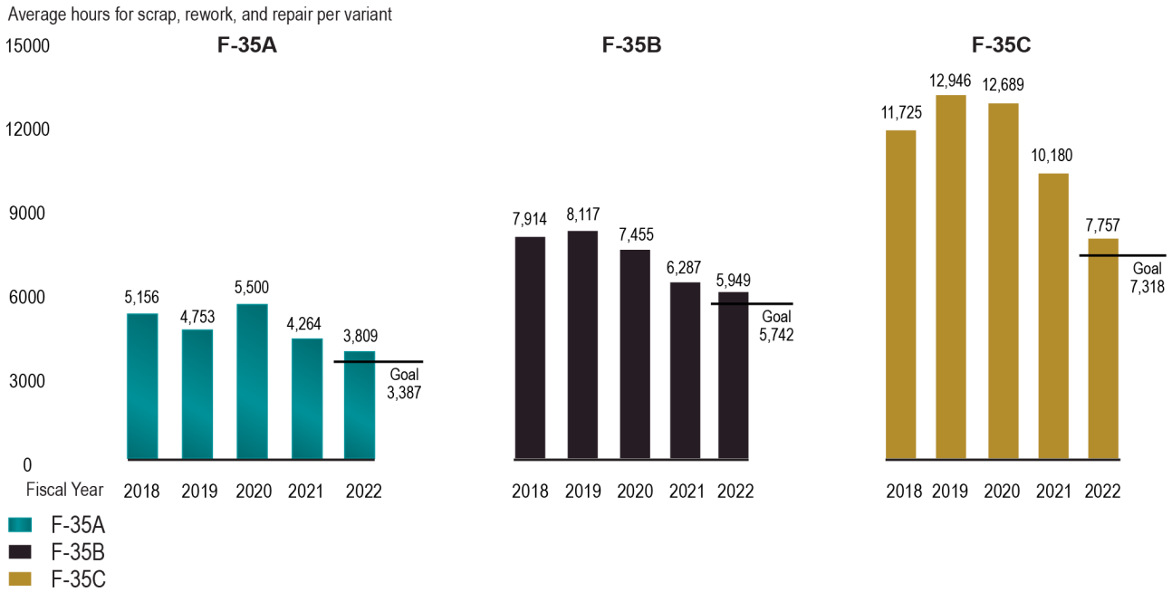
Figure 7: F-35 Airframe Contractor Scrap, Rework, and Repair Hours Improving but Still Not Meeting Goals
