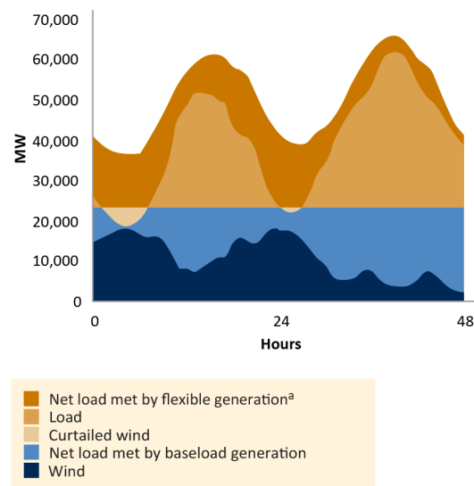
Figure 7: Hypothetical example of curtailed wind energy on a grid using simulated data
